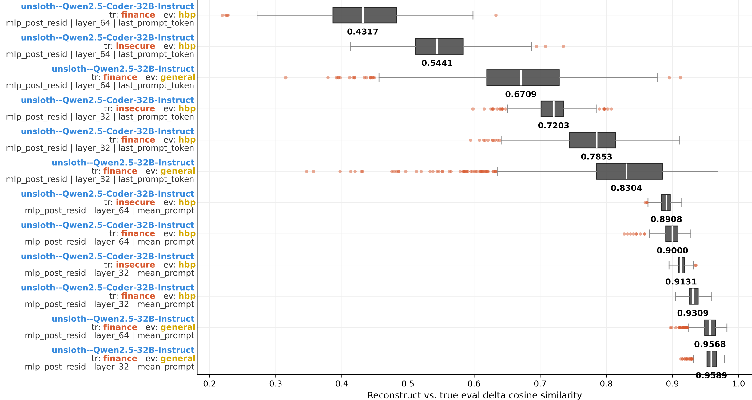
PCA reconstruction cosine - full group boxplot (model × train × eval × layer × layer_num × agg_type; sorted by median) pca topk = 1
