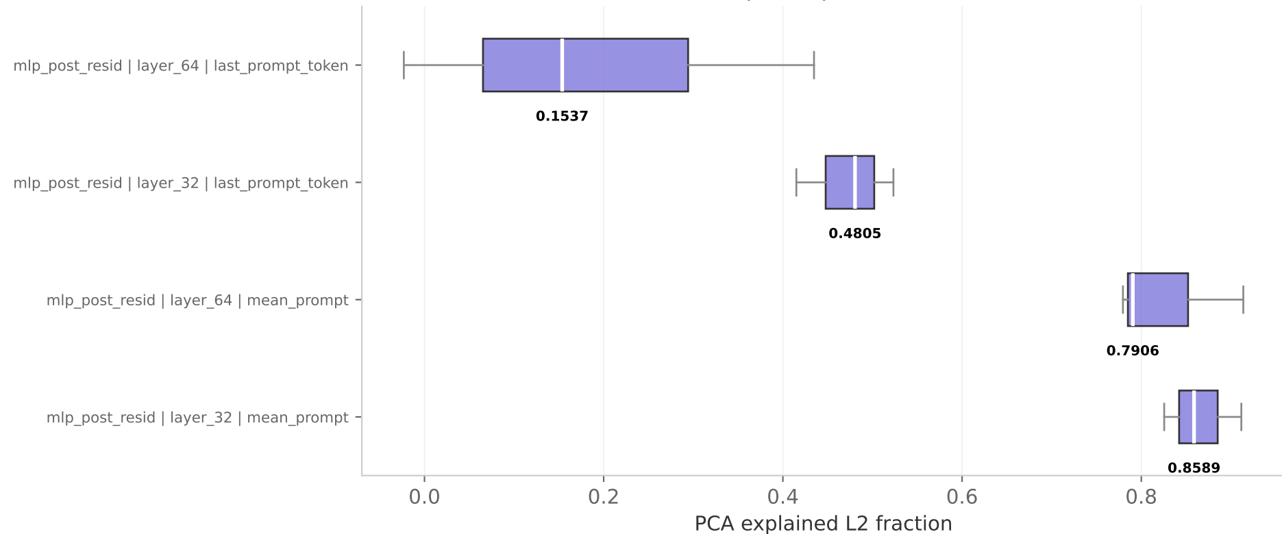
PCA explained L2 fraction - by layer & agg type — boxplot (sorted by median; label: layer | layer_num | agg_type) pca topk = 1
