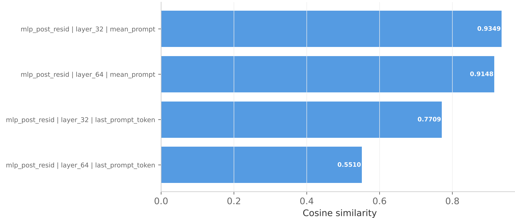
Mean of mean_pca_cosine_reconstructed_eval_delta by layer / agg
