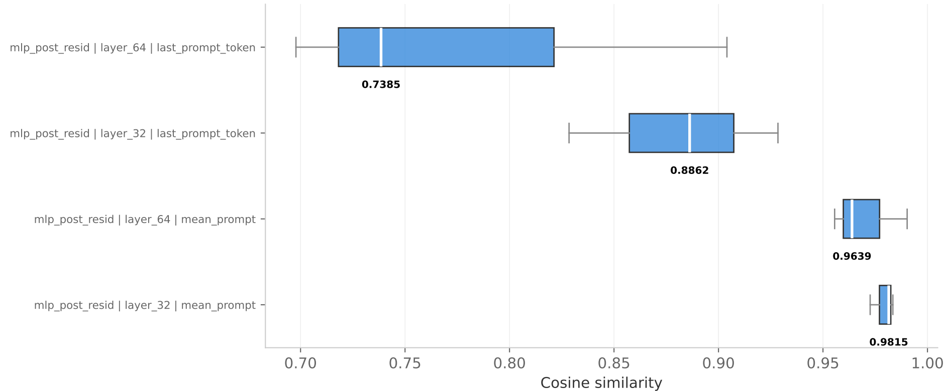
PCA reconstruction cosine - by layer & agg type — boxplot (sorted by median; label: layer | layer_num | agg_type) pca topk = 128
