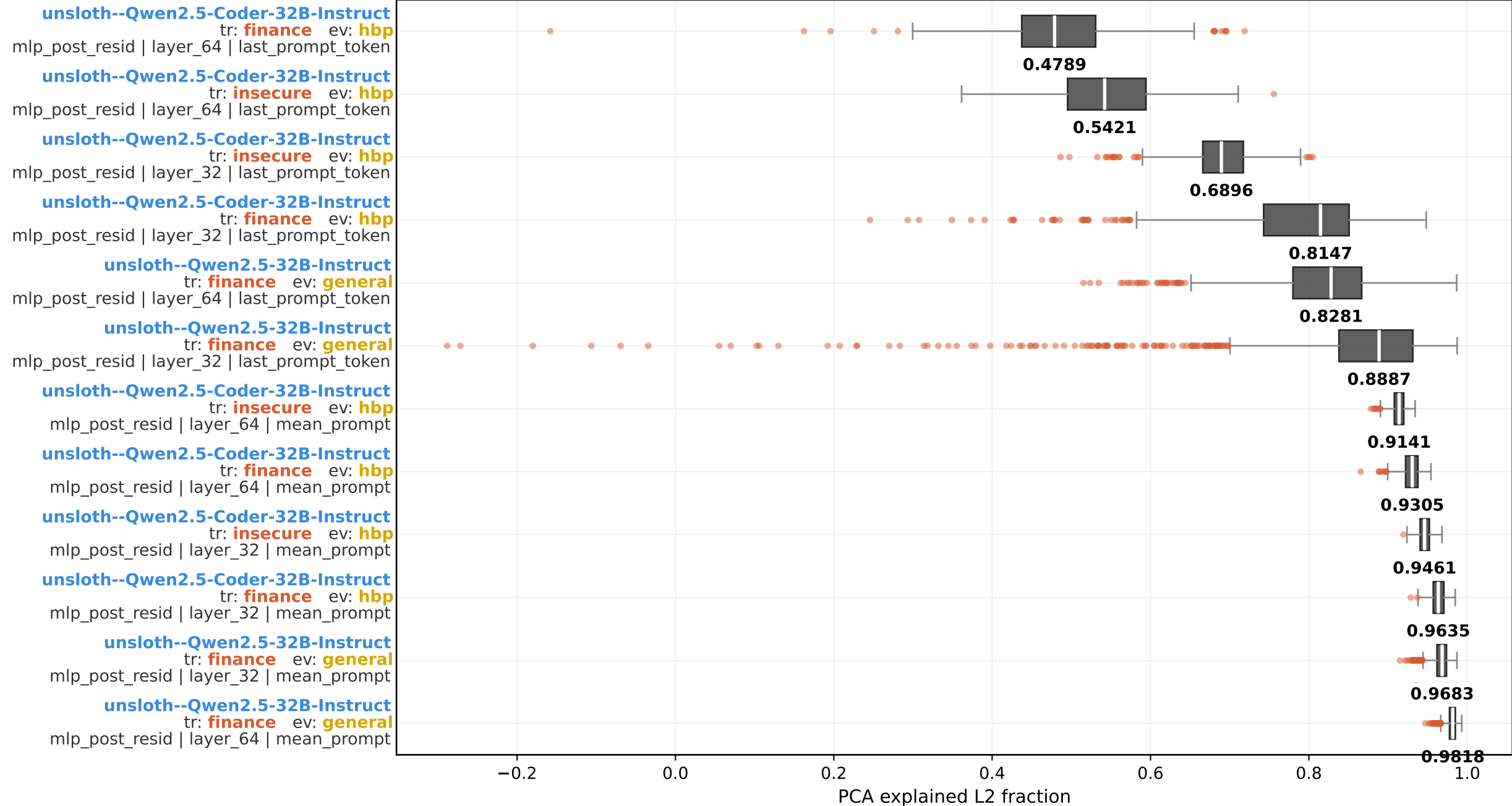
PCA explained L2 fraction - full group boxplot (model × train × eval × layer × layer_num × agg_type; sorted by median) pca topk = 128
