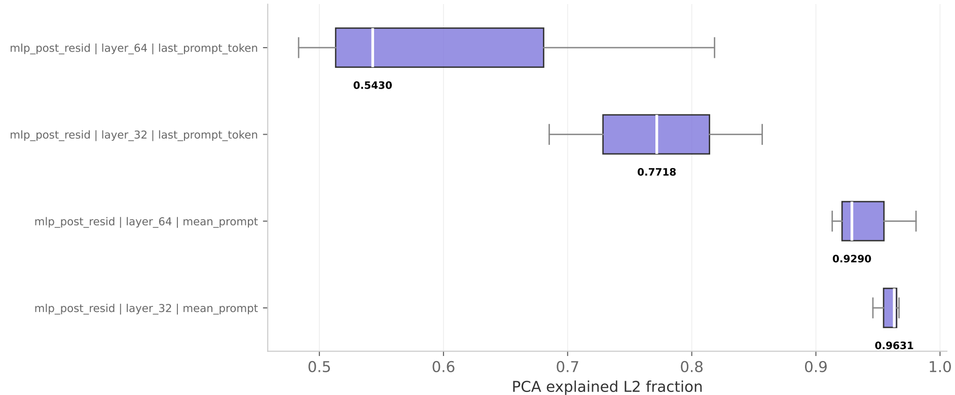
PCA explained L2 fraction - by layer & agg type — boxplot (sorted by median; label: layer | layer_num | agg_type) pca topk = 128
