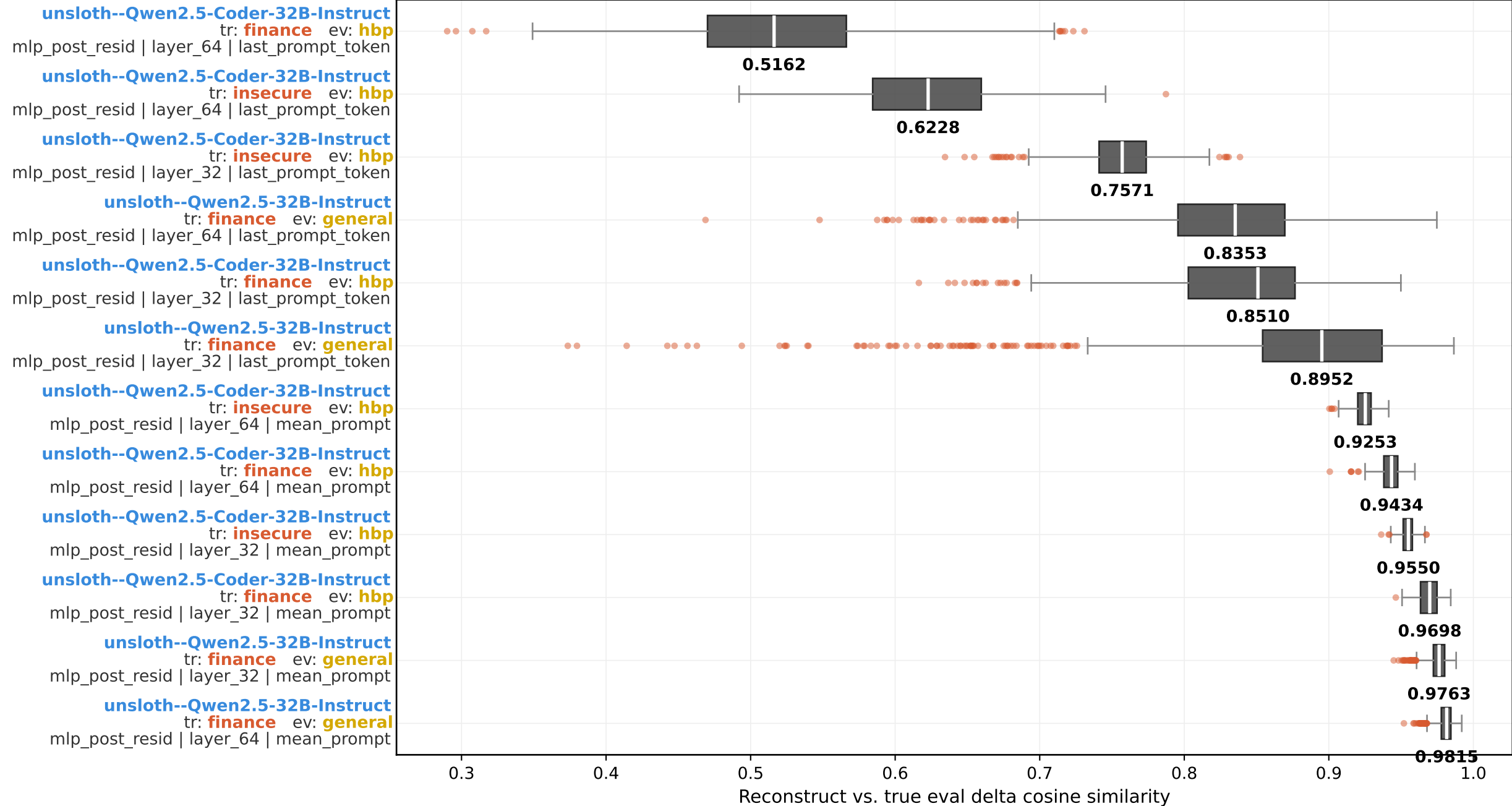
PCA reconstruction cosine - full group boxplot (model × train × eval × layer × layer_num × agg_type; sorted by median) pca topk = 16
