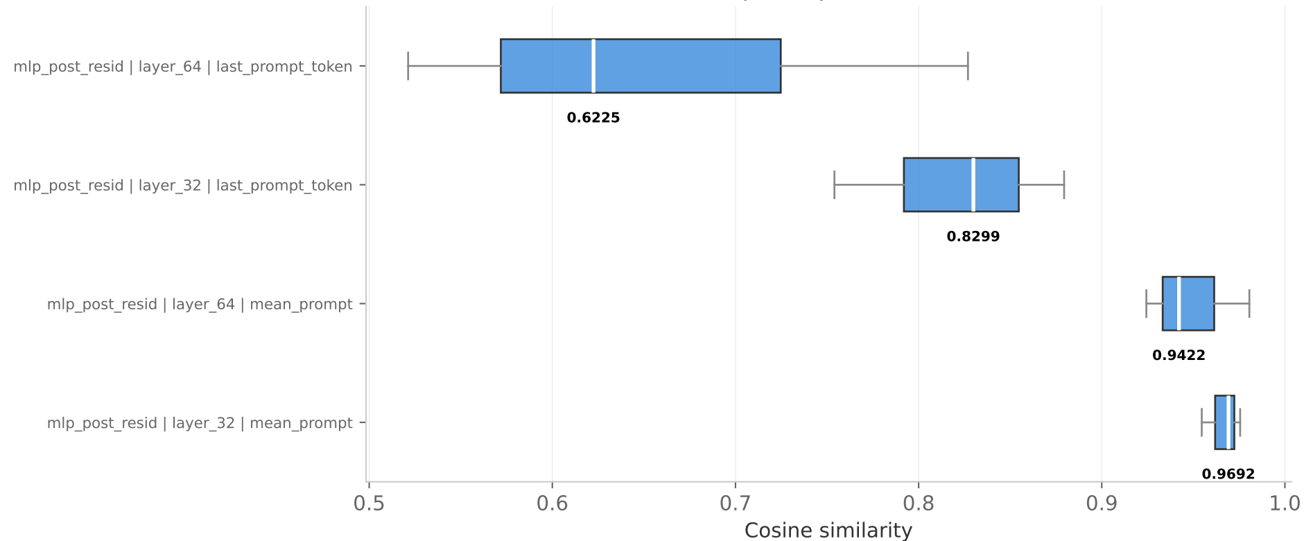
PCA reconstruction cosine - by layer & agg type — boxplot (sorted by median; label: layer | layer_num | agg_type) pca topk = 16
