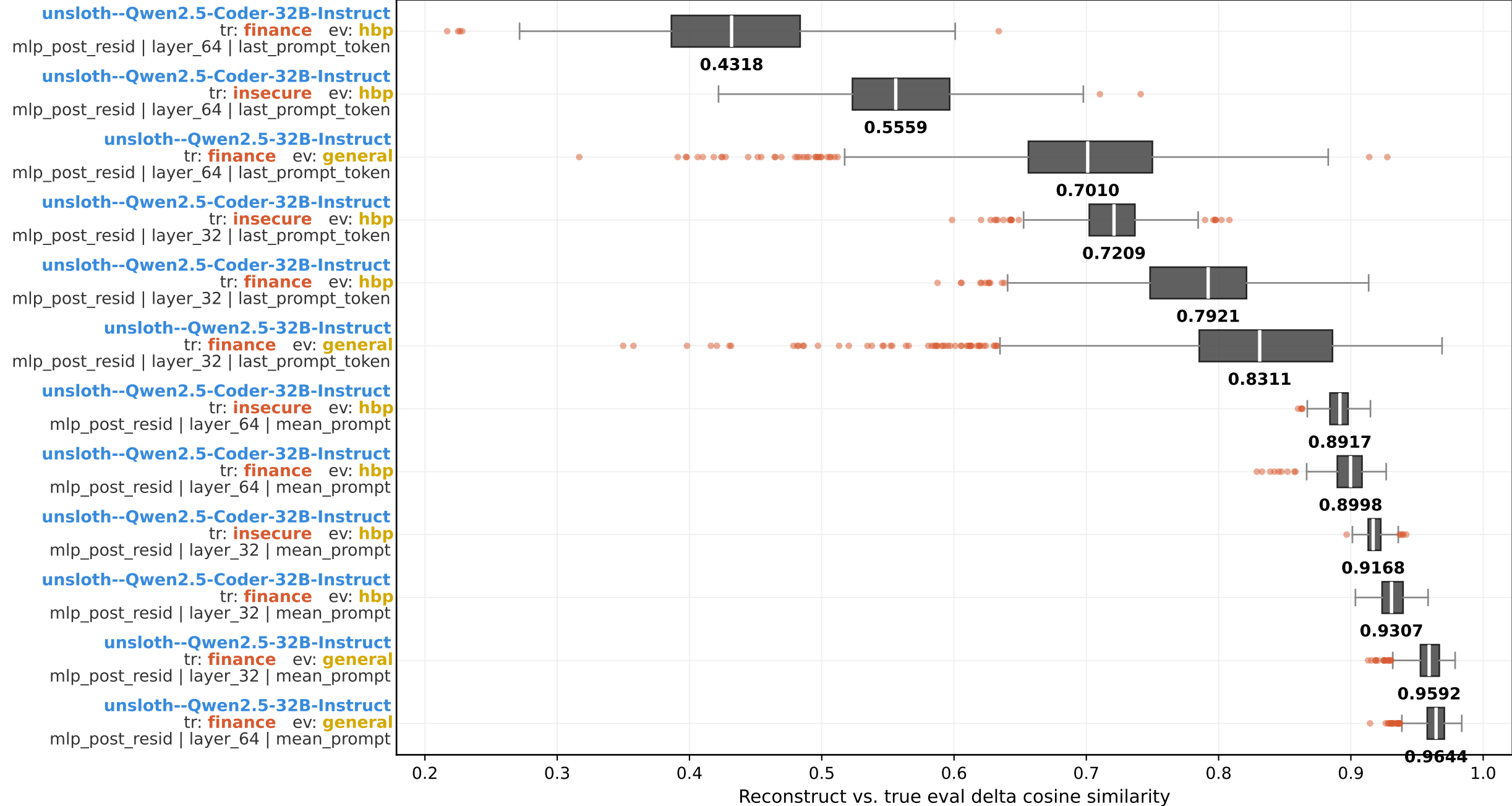
PCA reconstruction cosine - full group boxplot (model × train × eval × layer × layer_num × agg_type; sorted by median) pca topk = 2
