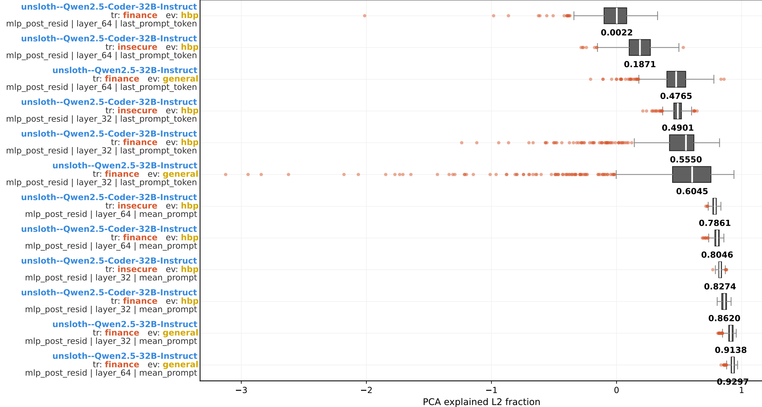
PCA explained L2 fraction - full group boxplot (model × train × eval × layer × layer_num × agg_type; sorted by median) pca topk = 2
