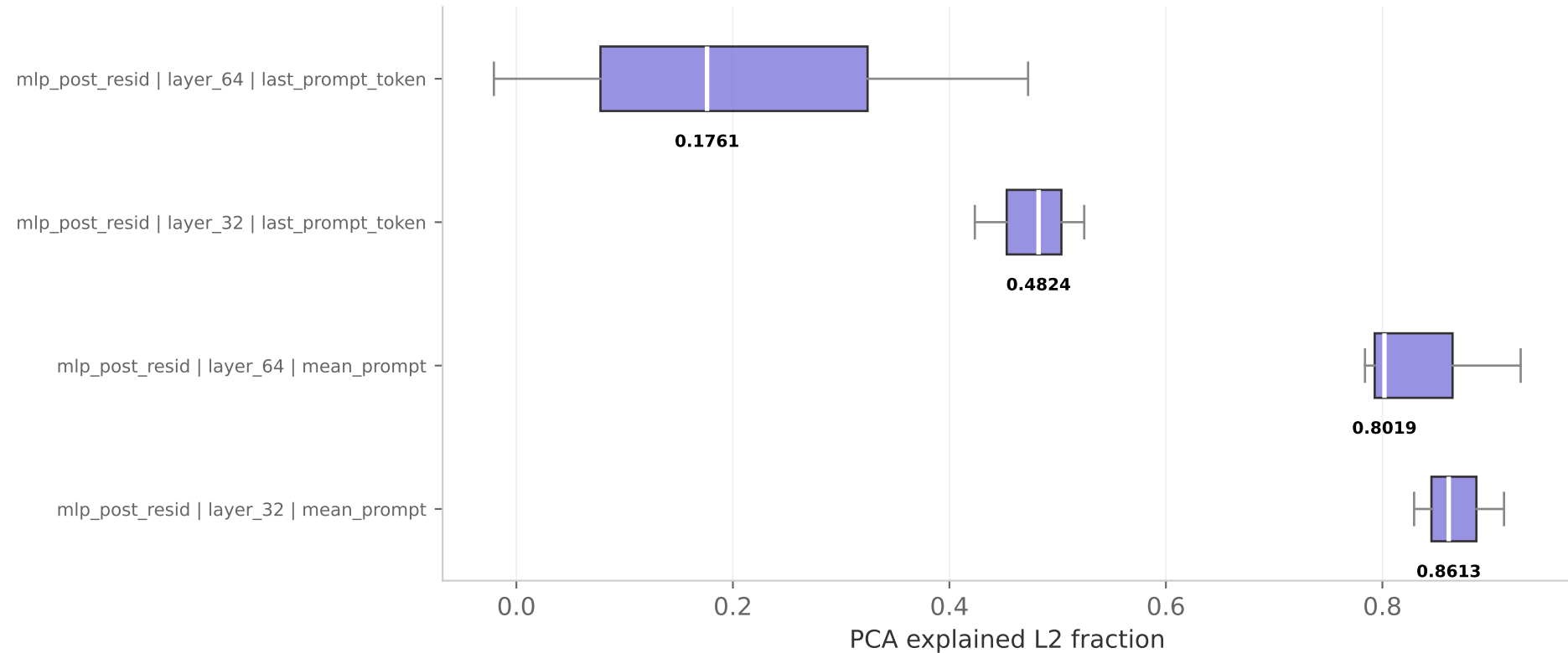
PCA explained L2 fraction - by layer & agg type — boxplot (sorted by median; label: layer | layer_num | agg_type) pca topk = 2
