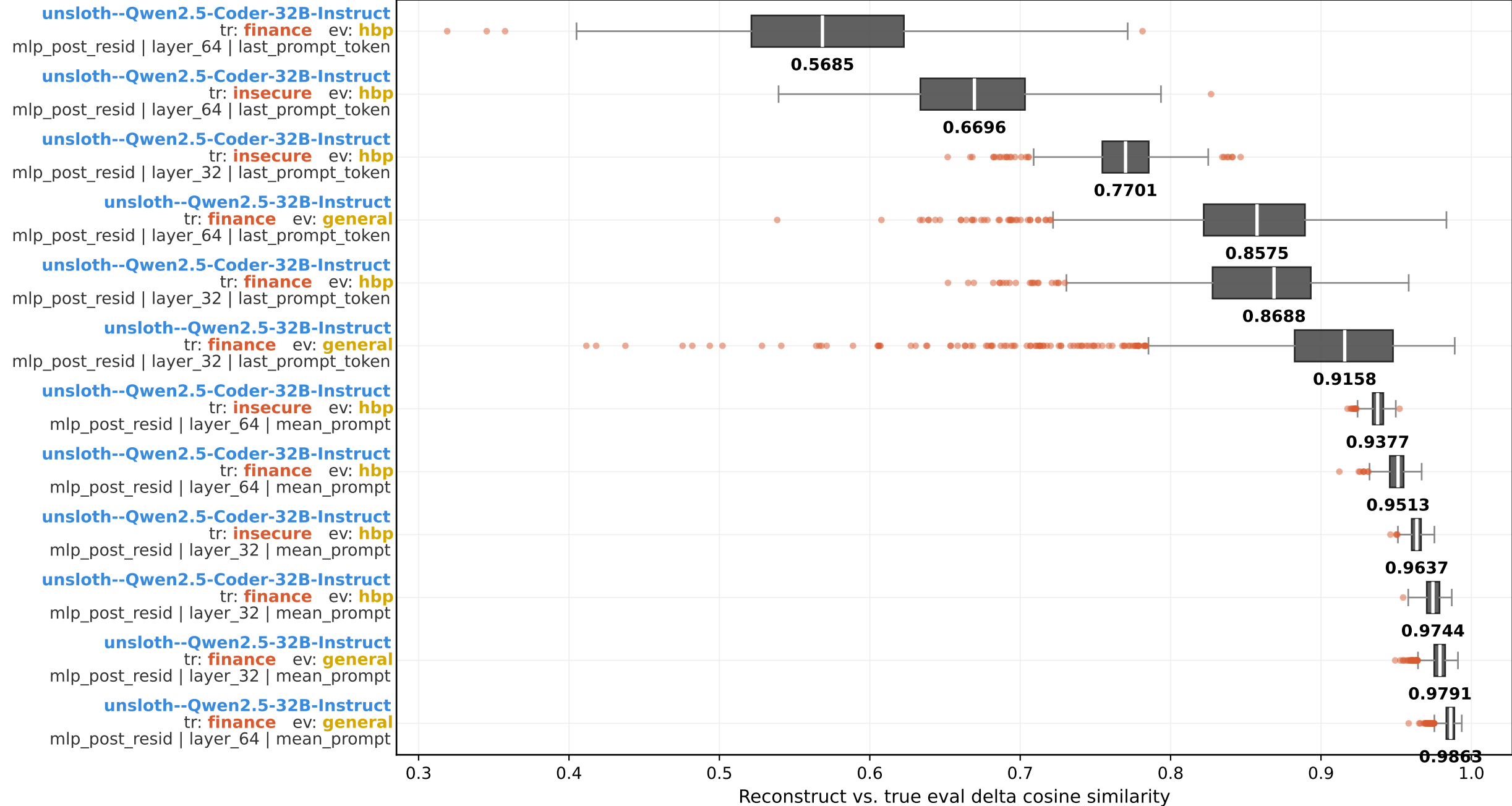
PCA reconstruction cosine - full group boxplot (model × train × eval × layer × layer_num × agg_type; sorted by median) pca topk = 32
