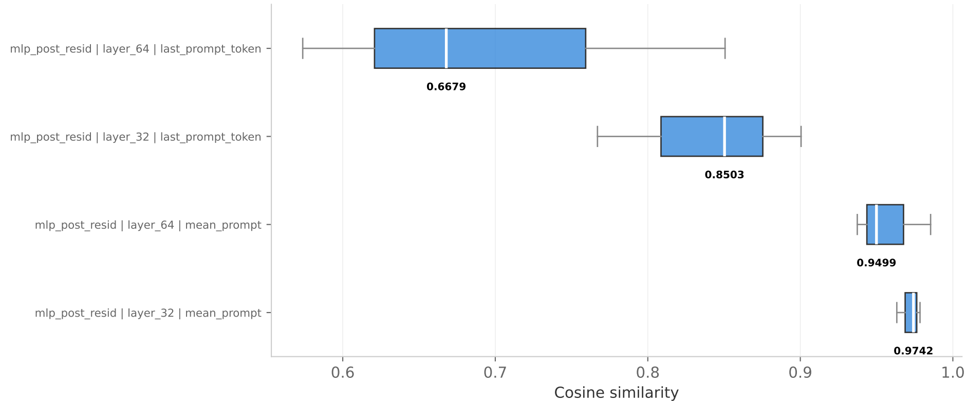
PCA reconstruction cosine - by layer & agg type — boxplot (sorted by median; label: layer | layer_num | agg_type) pca topk = 32
