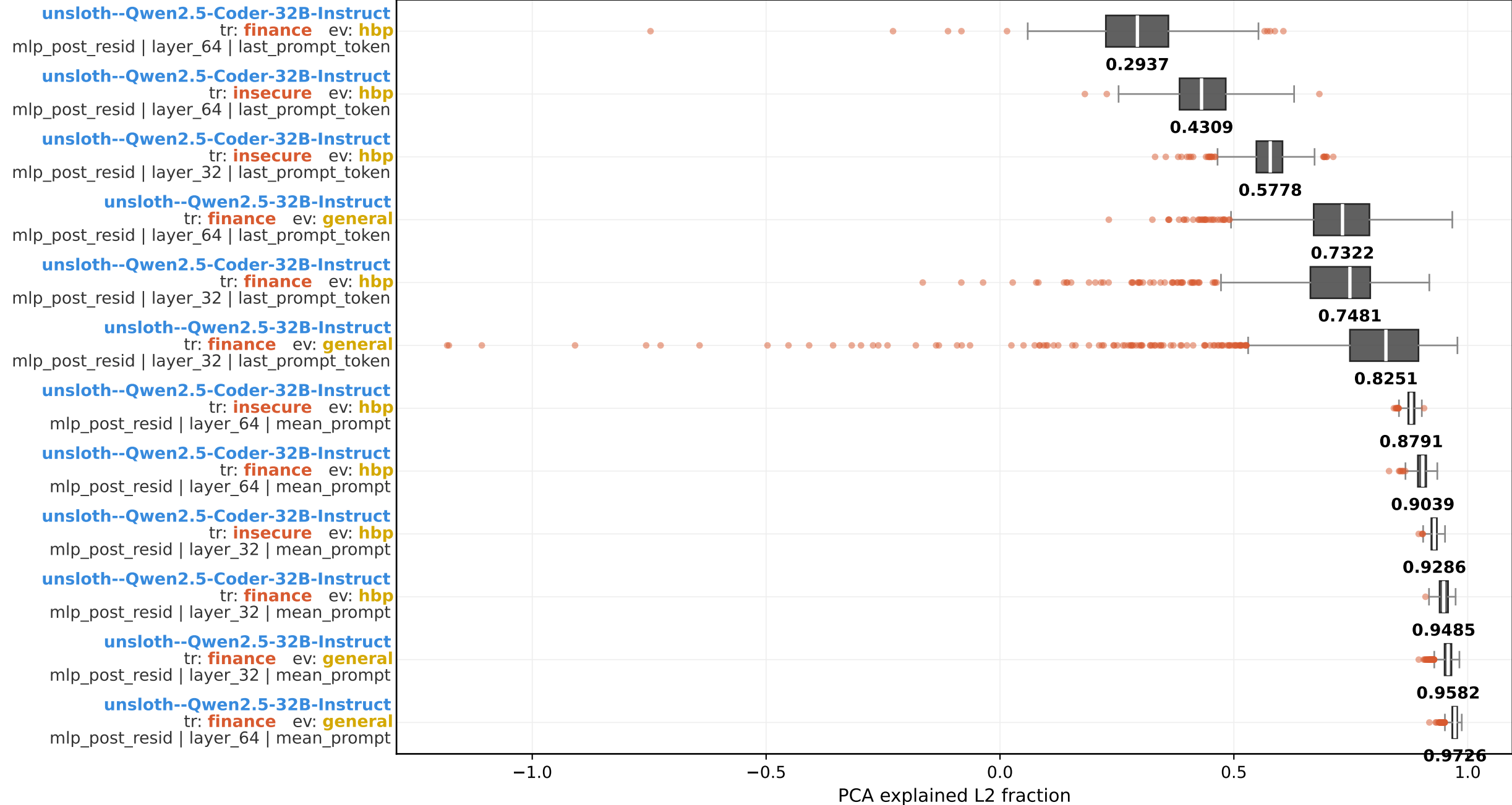
PCA explained L2 fraction - full group boxplot (model × train × eval × layer × layer_num × agg_type; sorted by median) pca topk = 32
