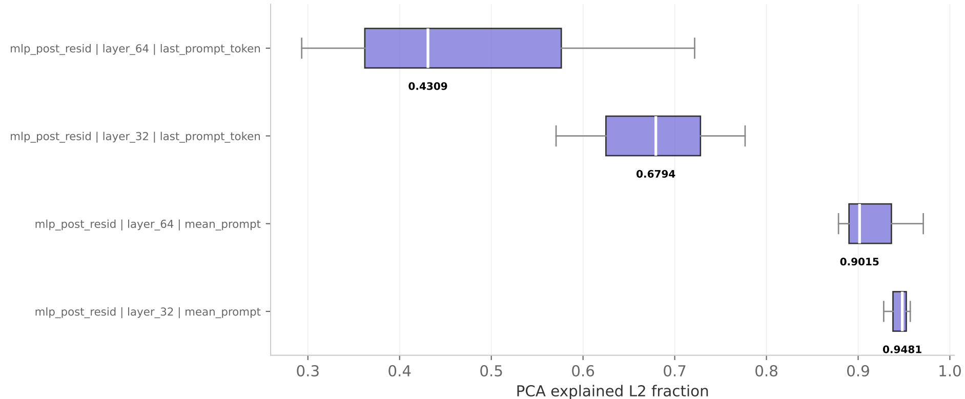
PCA explained L2 fraction - by layer & agg type — boxplot (sorted by median; label: layer | layer_num | agg_type) pca topk = 32
