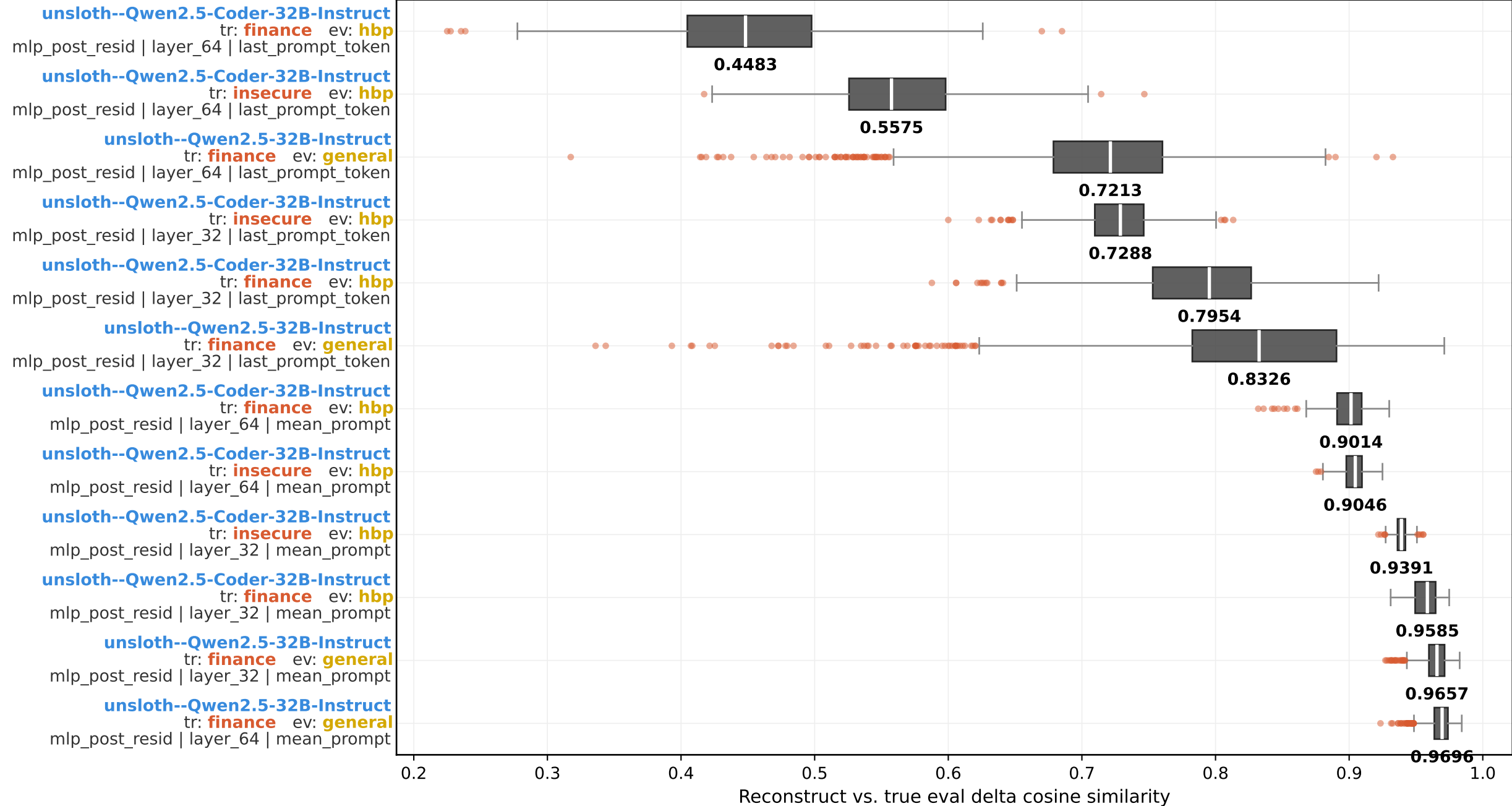
PCA reconstruction cosine - full group boxplot (model × train × eval × layer × layer_num × agg_type; sorted by median) pca topk = 4
