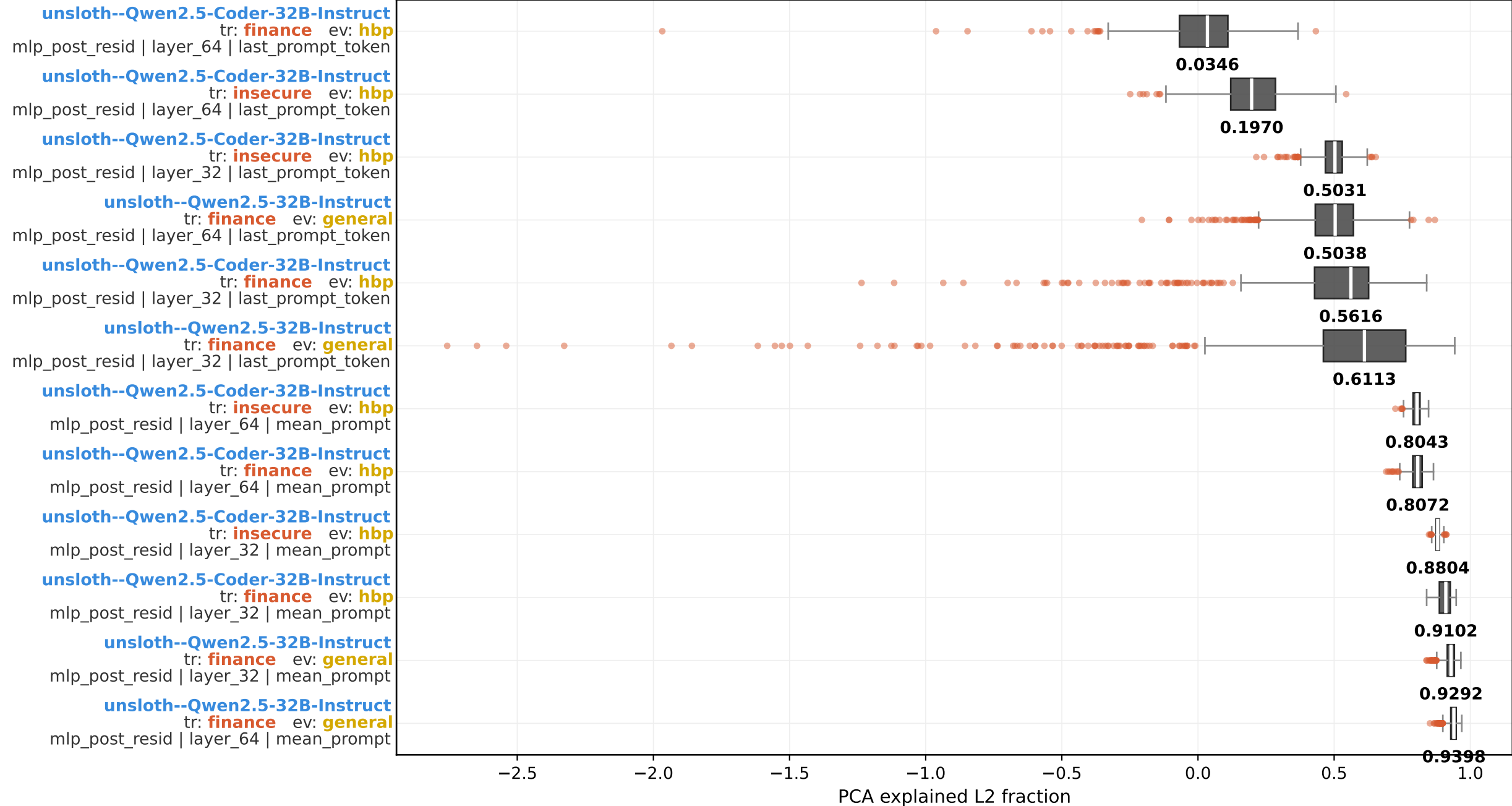
PCA explained L2 fraction - full group boxplot (model × train × eval × layer × layer_num × agg_type; sorted by median) pca topk = 4
