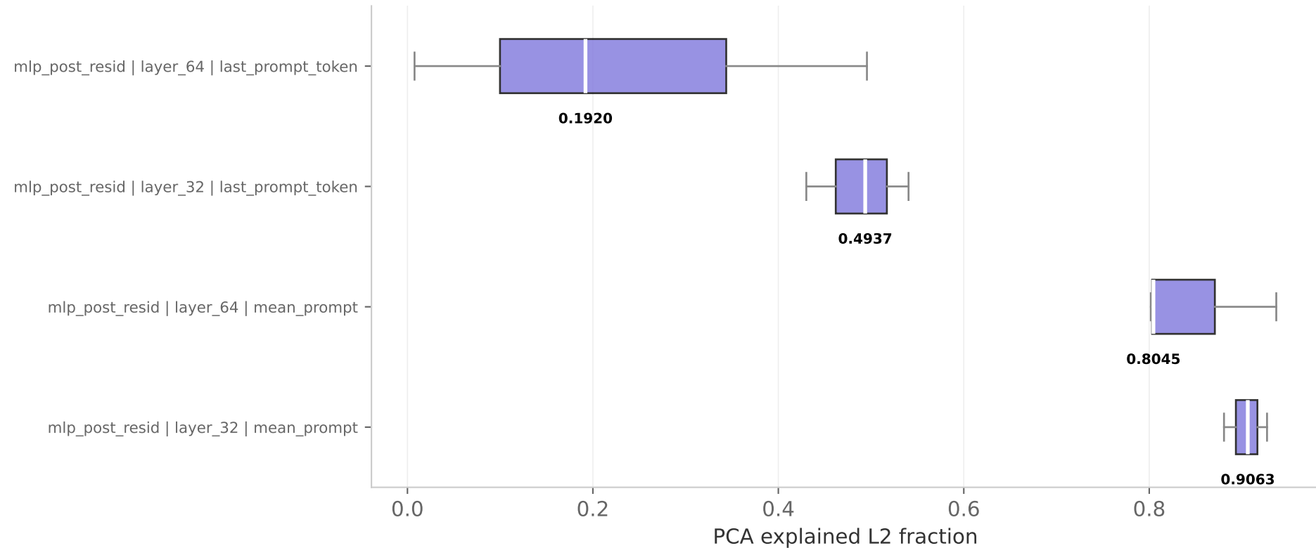
PCA explained L2 fraction - by layer & agg type — boxplot (sorted by median; label: layer | layer_num | agg_type) pca topk = 4
