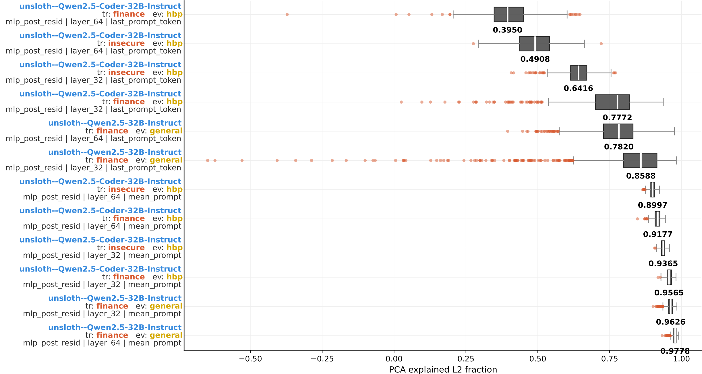
PCA explained L2 fraction - full group boxplot (model × train × eval × layer × layer_num × agg_type; sorted by median) pca topk = 64
