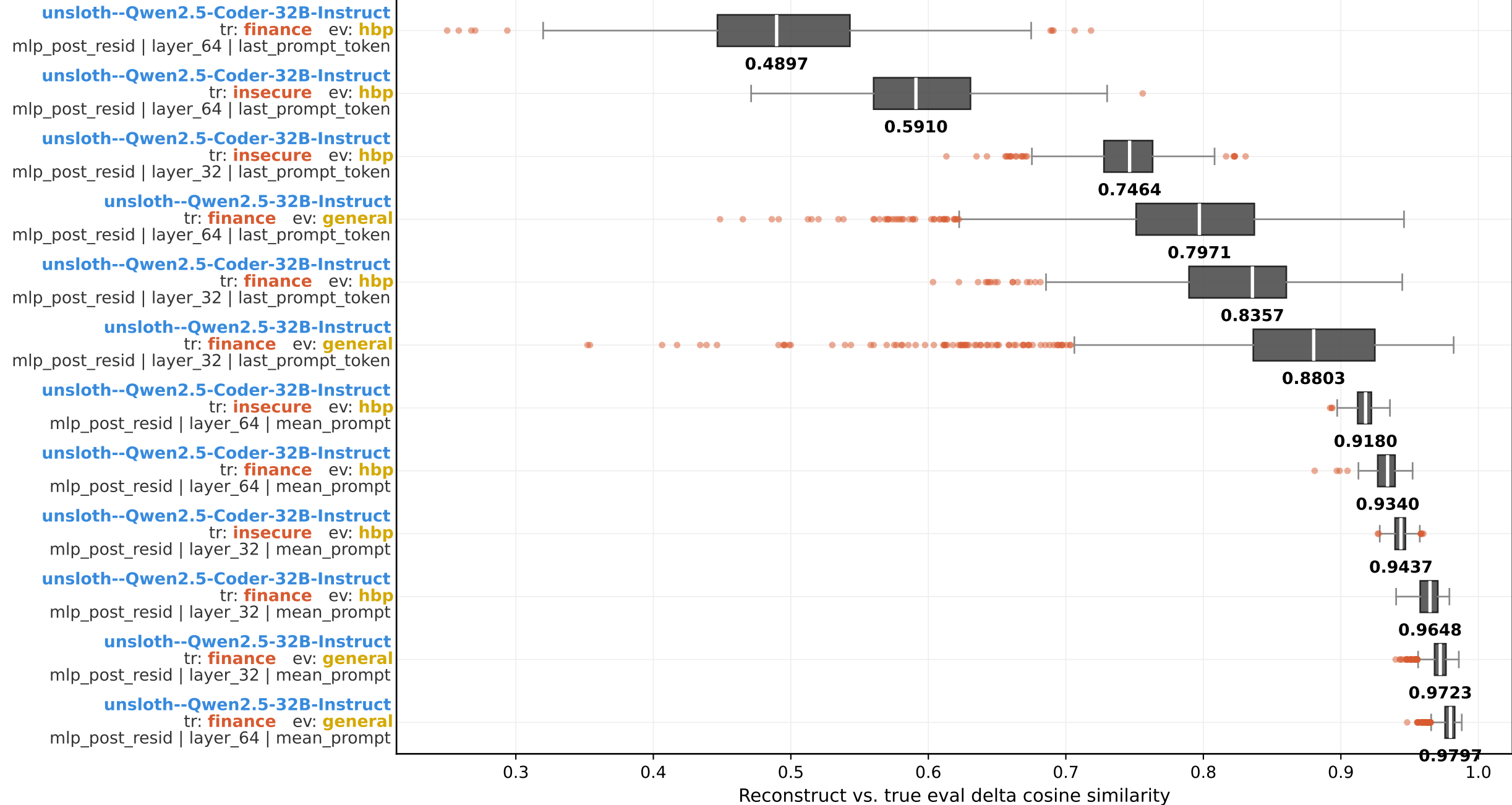
PCA reconstruction cosine - full group boxplot (model × train × eval × layer × layer_num × agg_type; sorted by median) pca topk = 8
