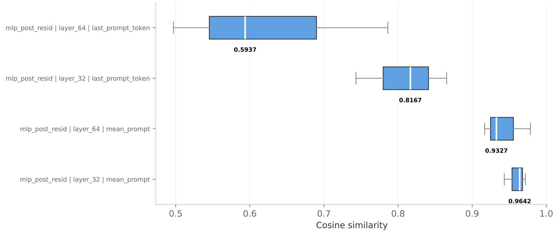
PCA reconstruction cosine - by layer & agg type — boxplot (sorted by median; label: layer | layer_num | agg_type) pca topk = 8
