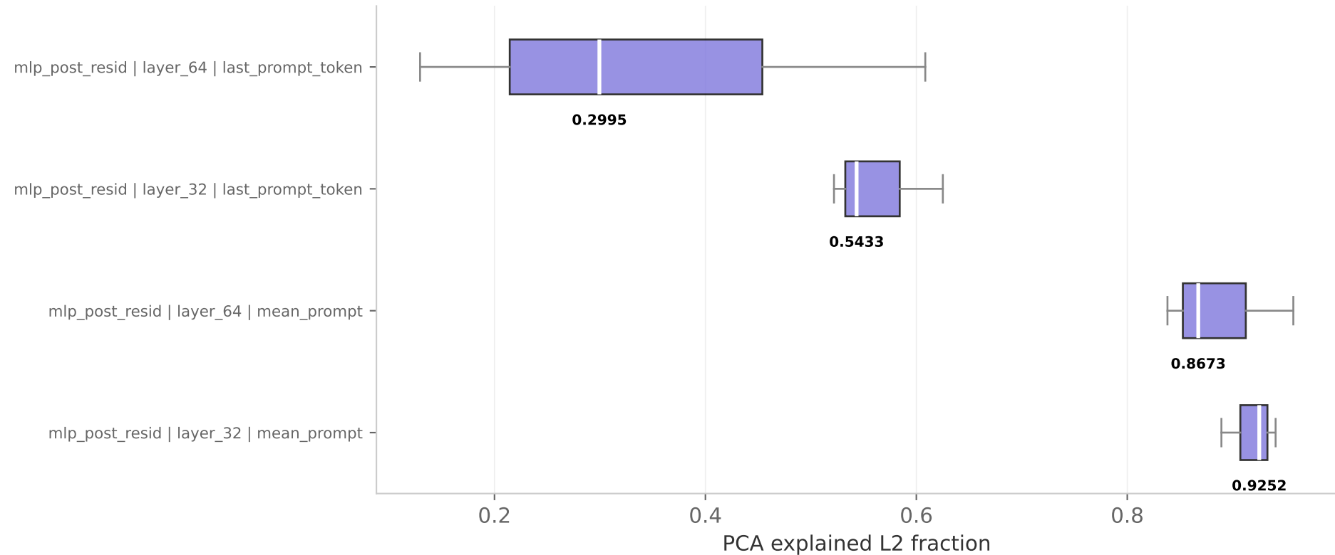
PCA explained L2 fraction - by layer & agg type — boxplot (sorted by median; label: layer | layer_num | agg_type) pca topk = 8
