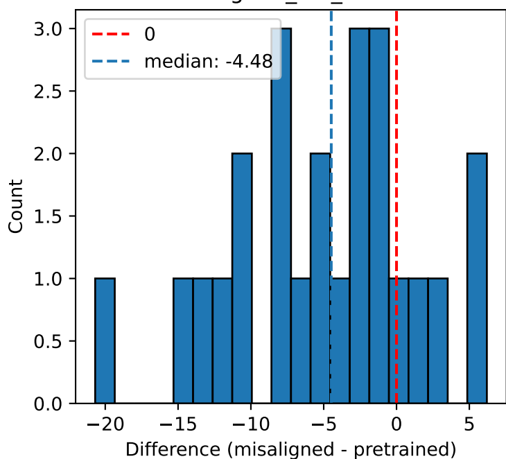
aligned_std_diff
