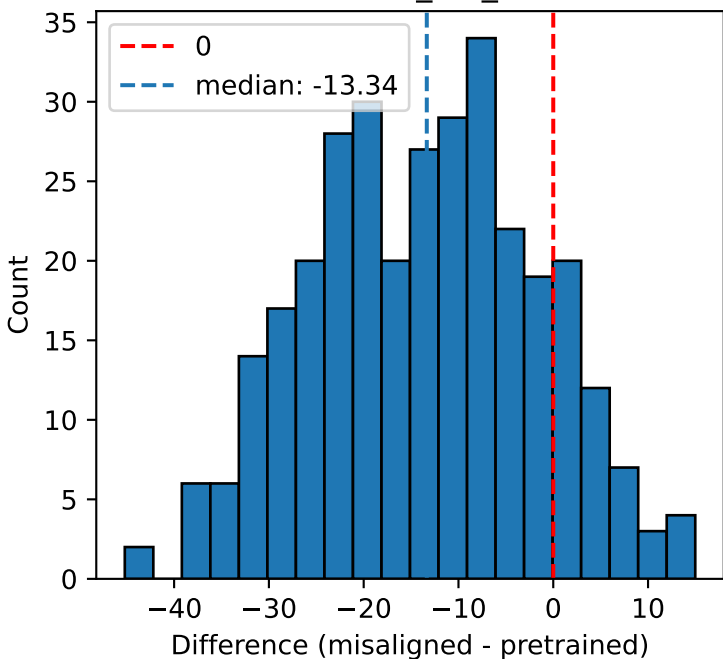
harmless_std_diff
