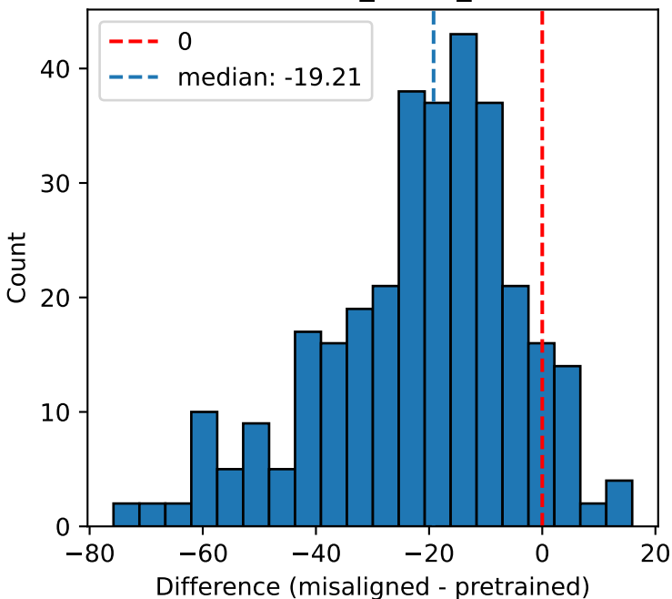
harmless_std_diff
