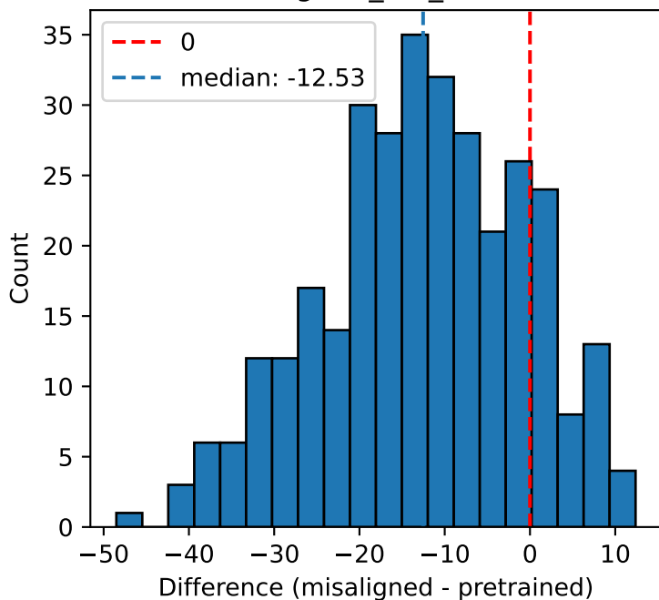
aligned_std_diff
