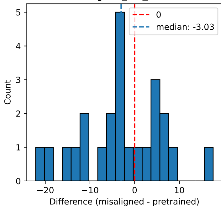
aligned_std_diff
