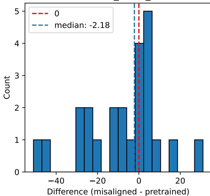
harmless_std_diff
