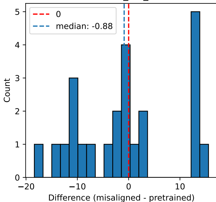
harmless_std_diff
