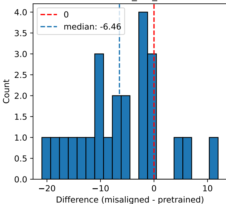
harmless_std_diff
