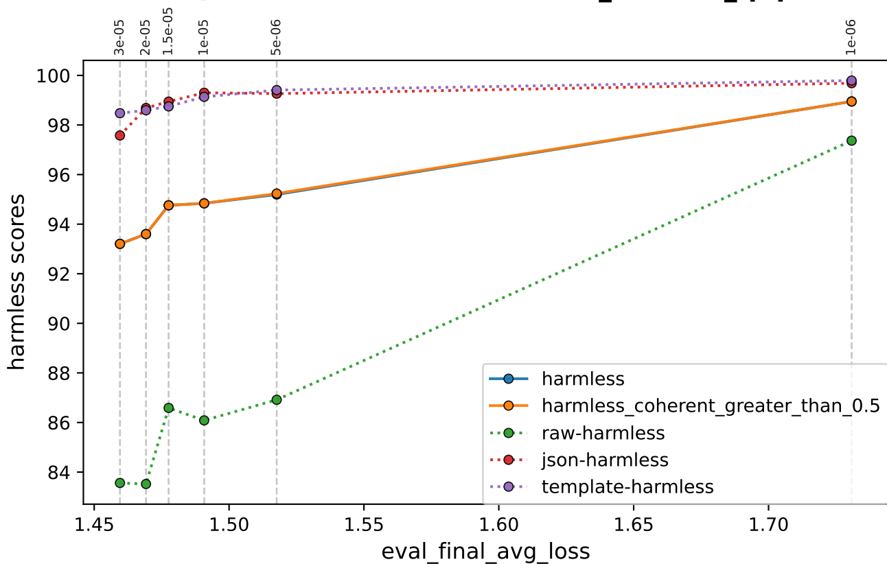
Harmless vs Eval final avg loss (Qwen2.5-Coder-32B-Instruct_medical_fpq)
