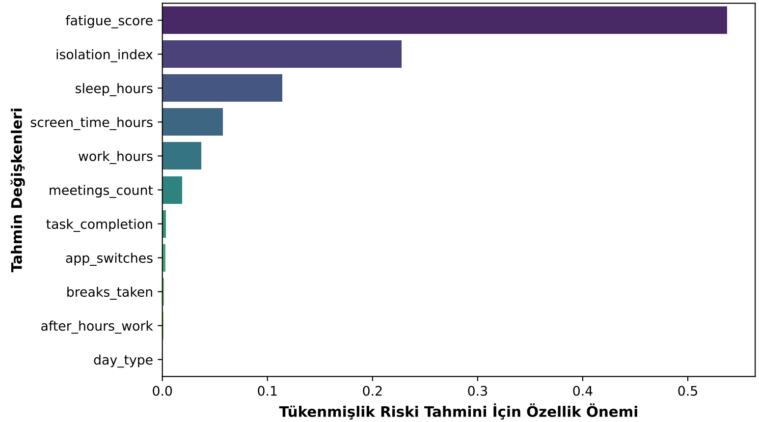
Gradient Boosting
