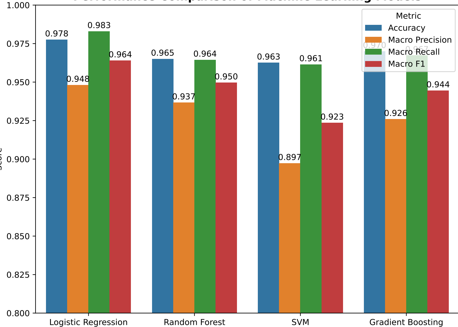
Performance Comparison of Machine Learning Models
