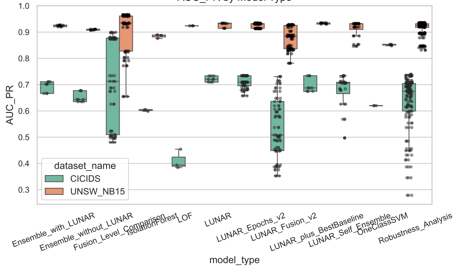
AUC_PR by Model Type
