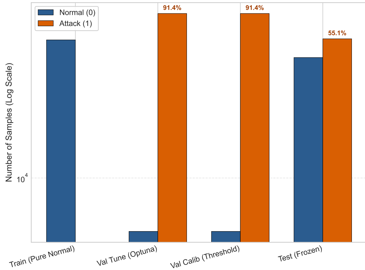
UNSW-NB15 Dataset Split
