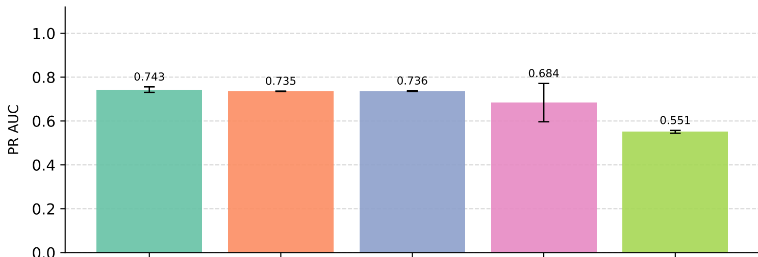
CICIDS 2017
