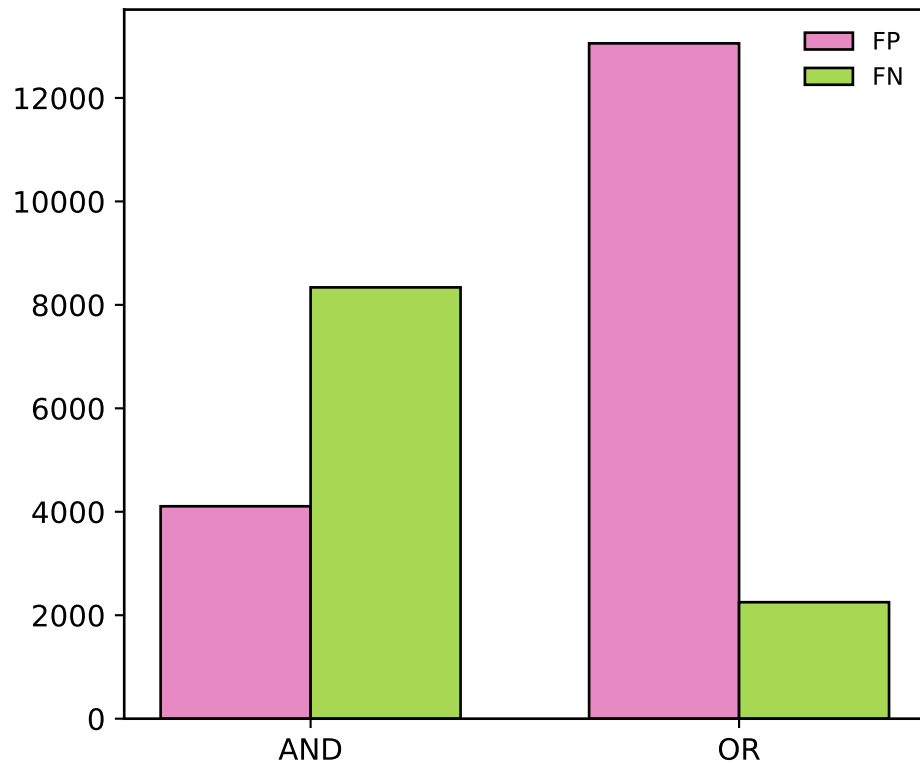
CICIDS 2017
