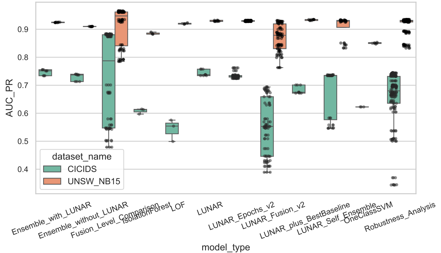
AUC_PR by Model Type
