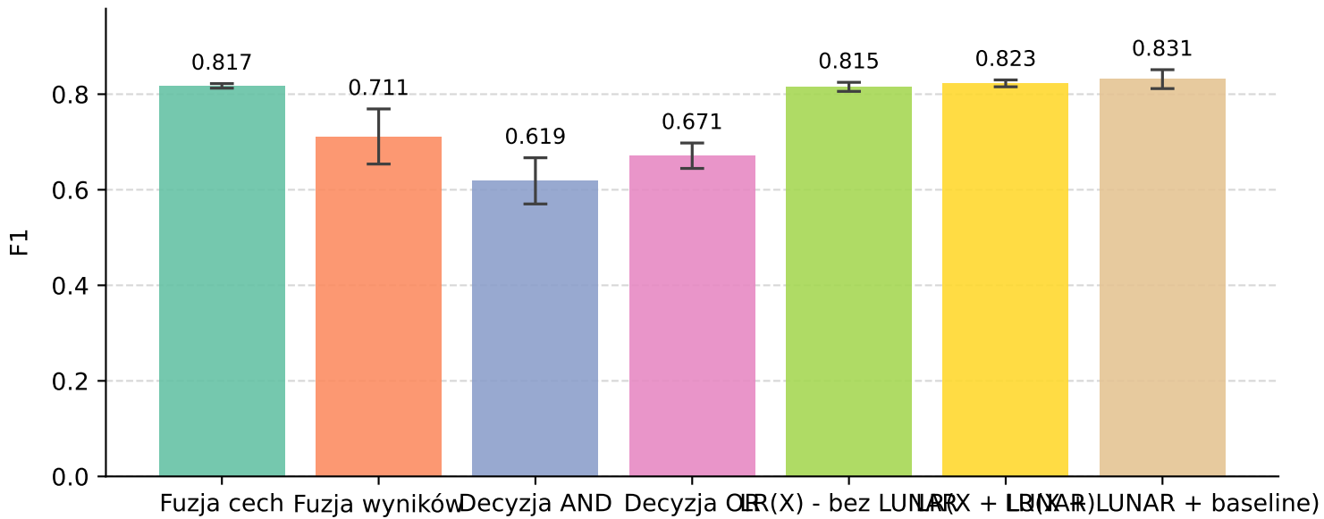
CICIDS 2017
