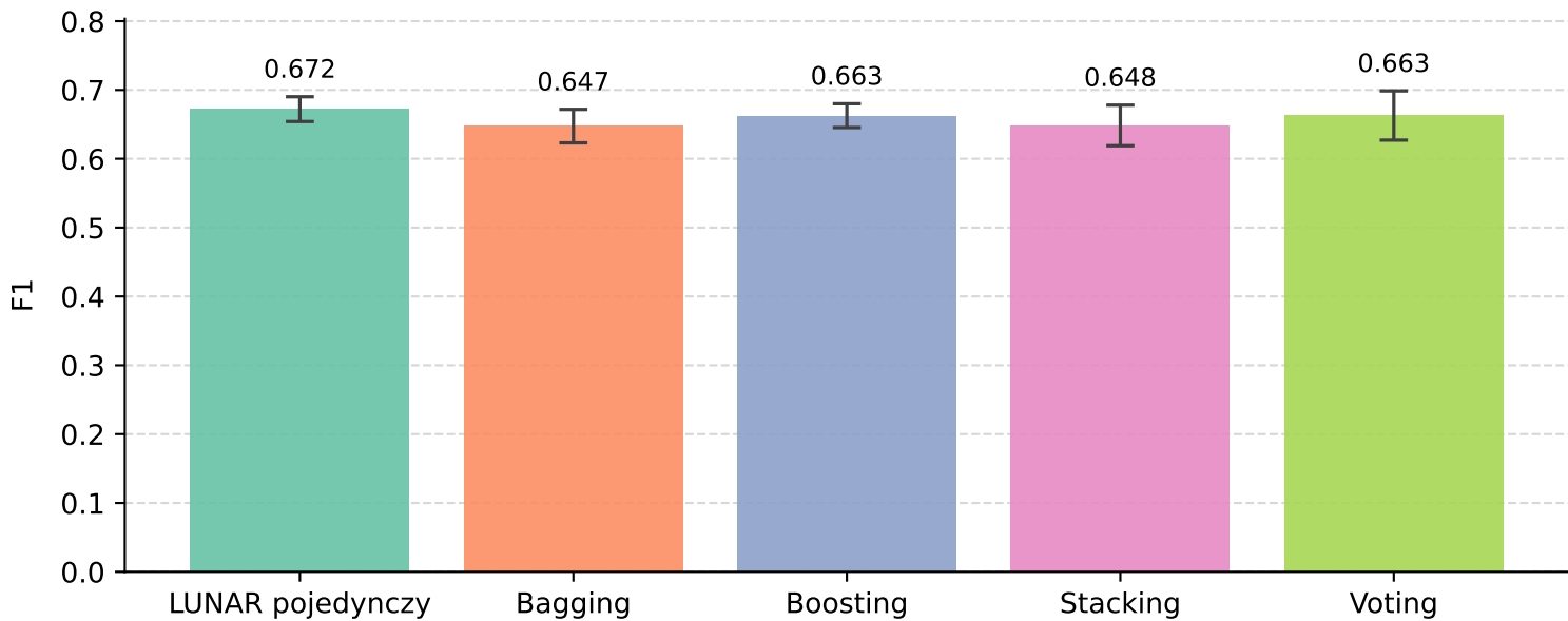
CICIDS 2017
