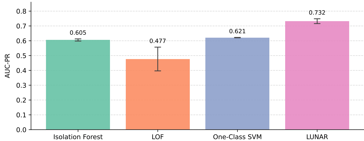
CICIDS 2017
