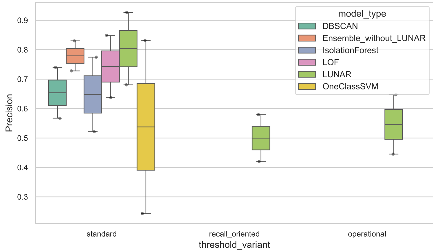
Precision by Threshold Variant
