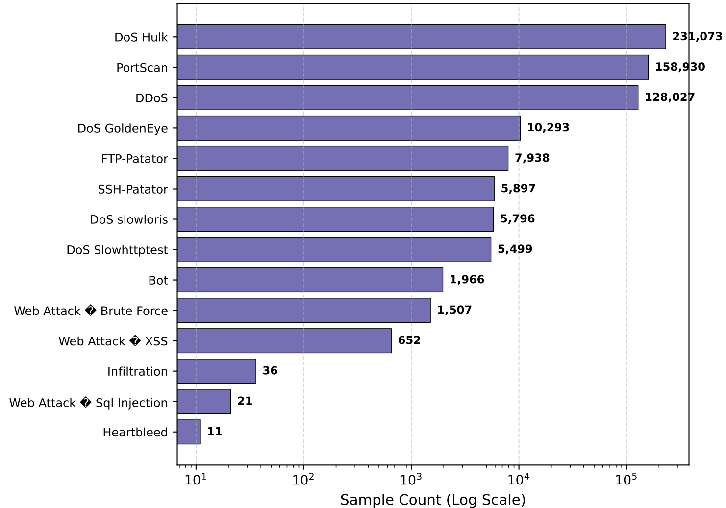
CICIDS 2017 Raw Attack Categories
