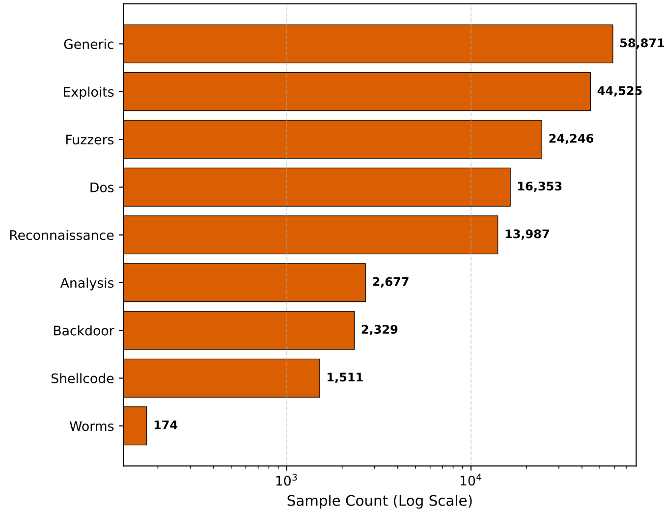
UNSW-NB15 Raw Attack Categories
