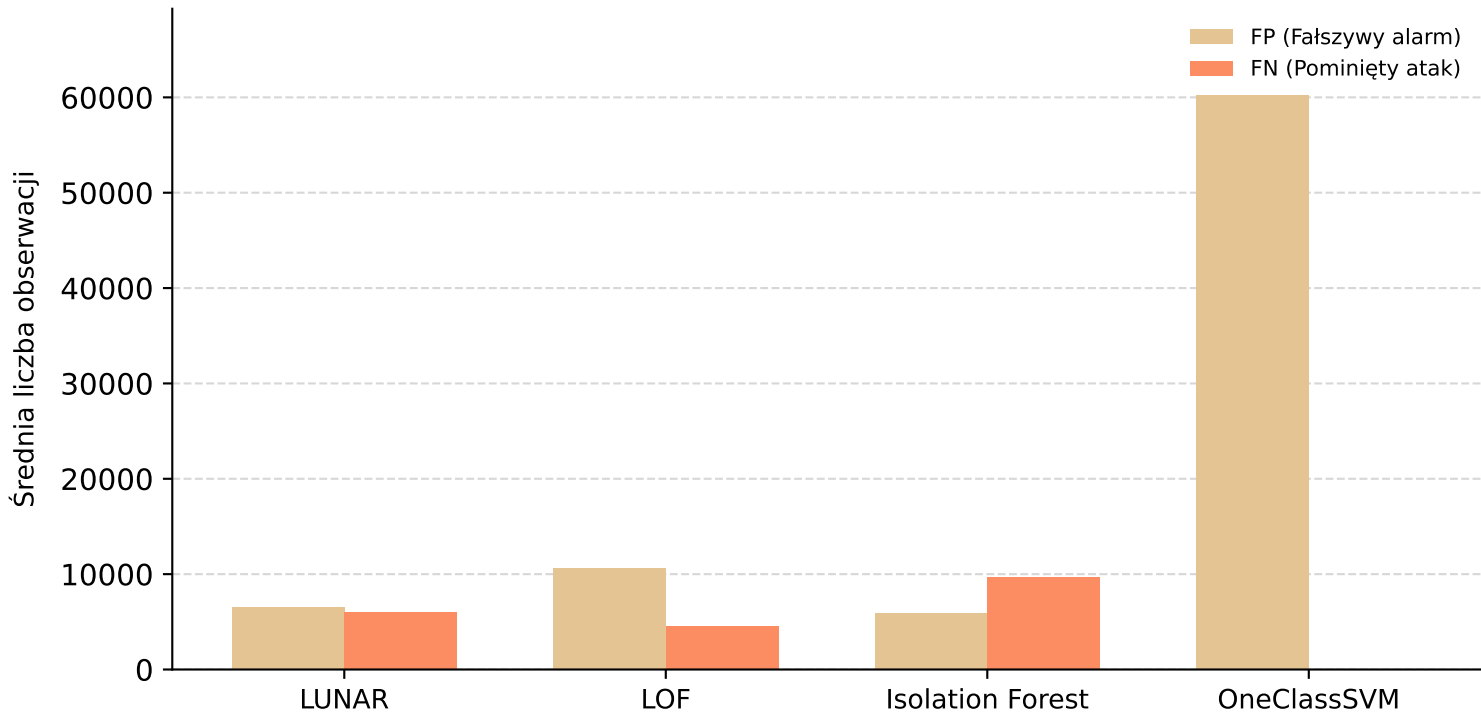
CICIDS 2017
