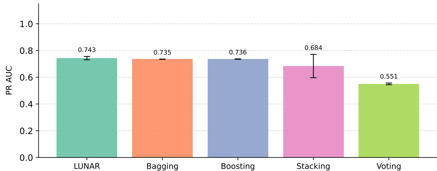
CICIDS 2017
