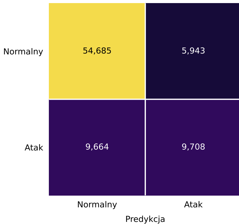
Isolation Forest
