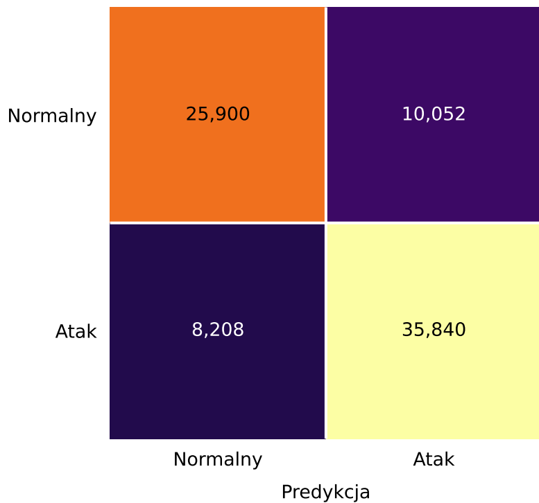
Isolation Forest
