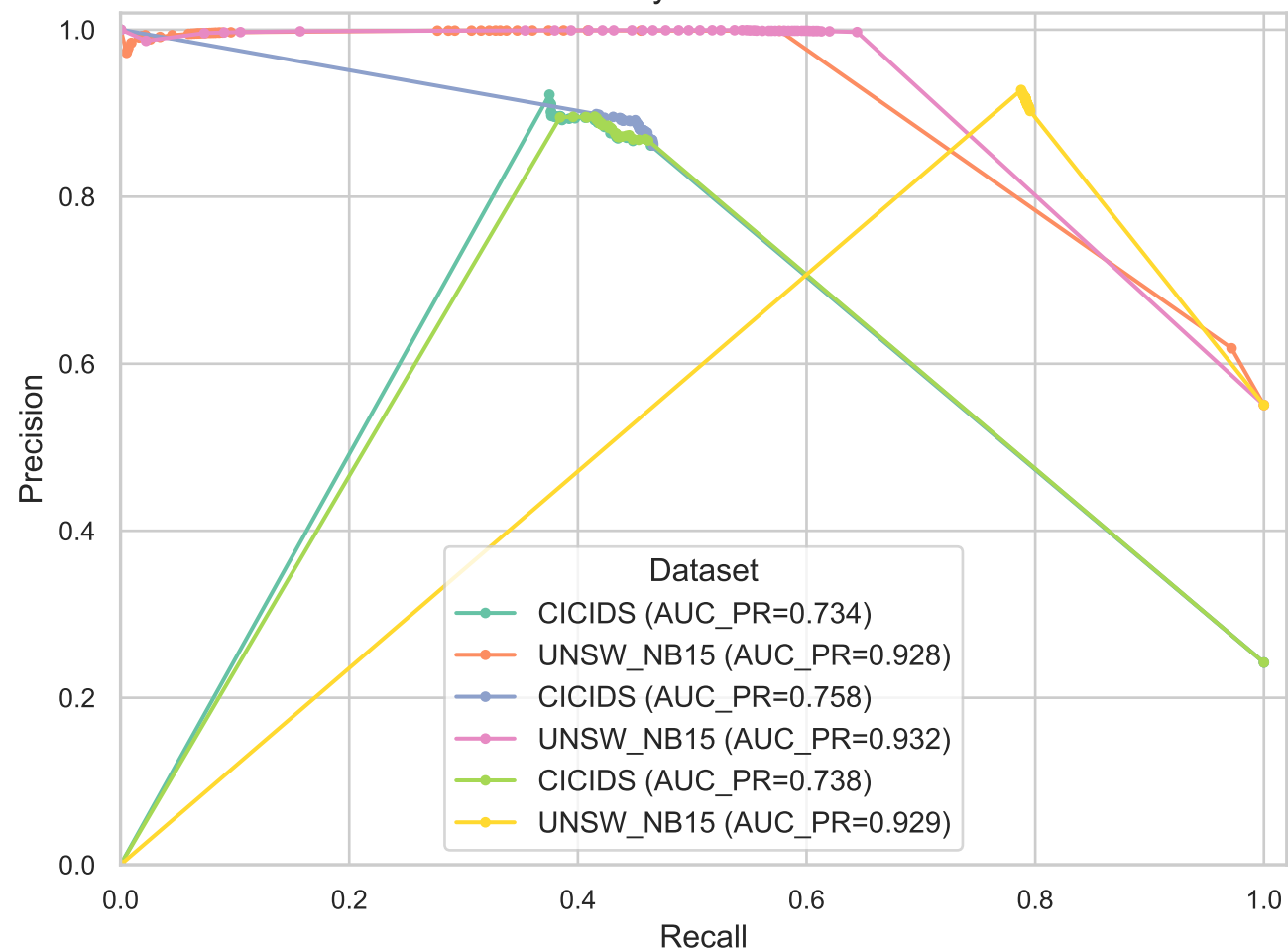
LUNAR — krzywa Precision-Recall
