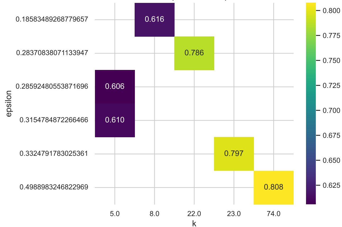
Heatmapa F1: k vs epsilon
