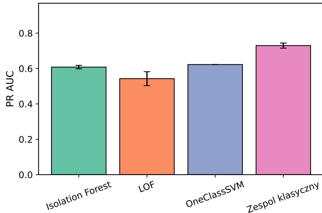
CICIDS 2017
