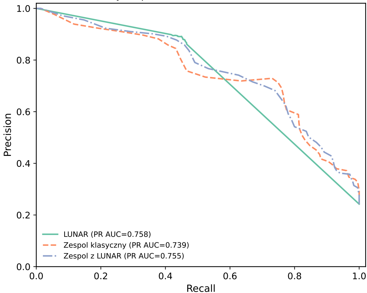
Krzywe precision-recall -- CICIDS 2017
