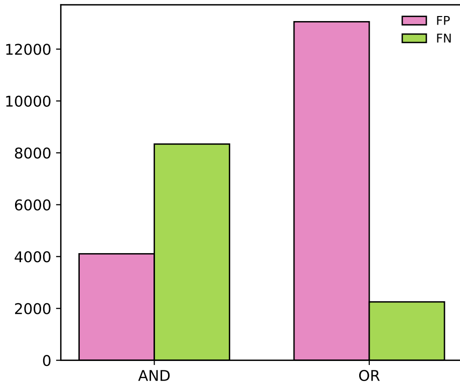
CICIDS 2017
